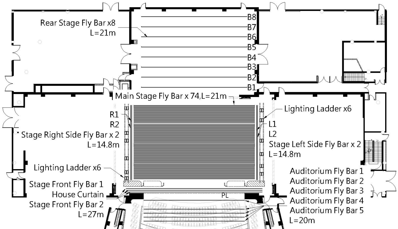
Figure 1.3.1- Rigging Plan
