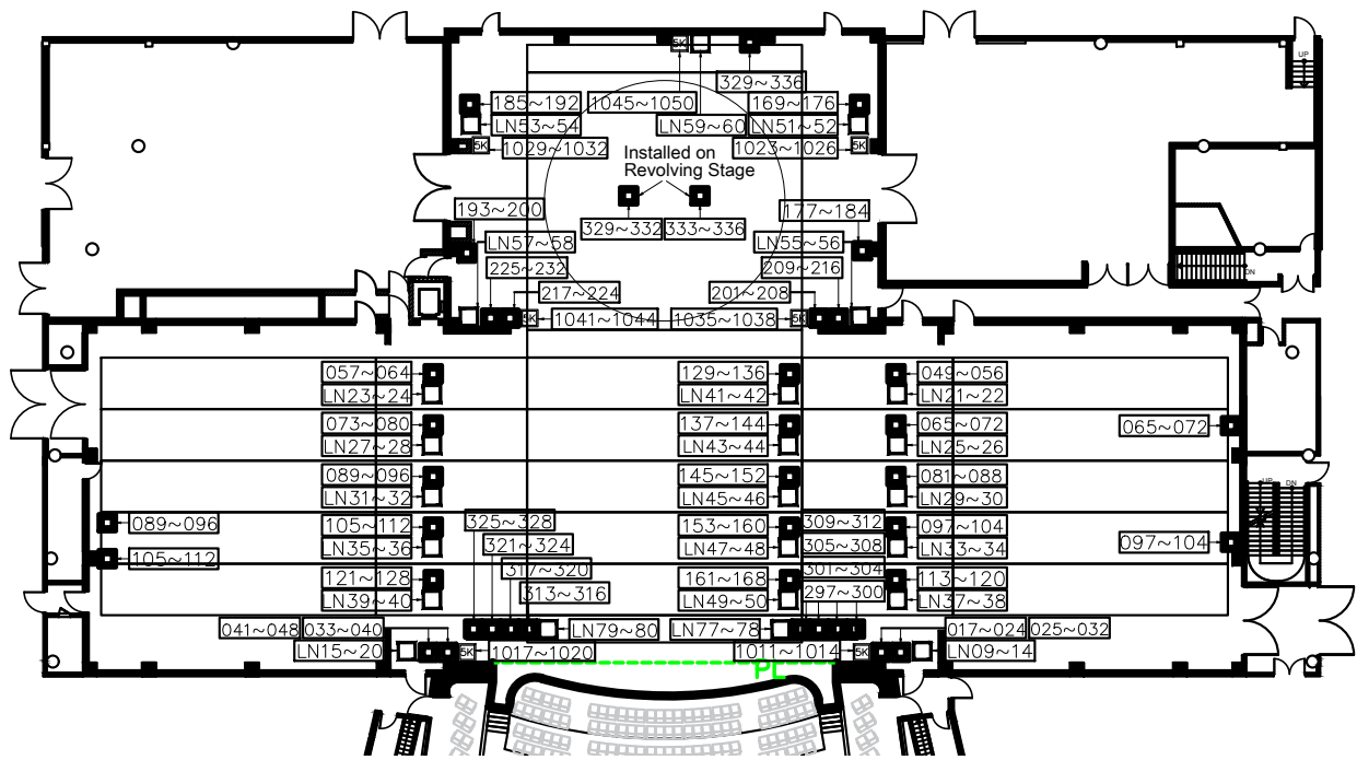
Figure 2.3.1.1- First Floor Lighting Circuit Layout
