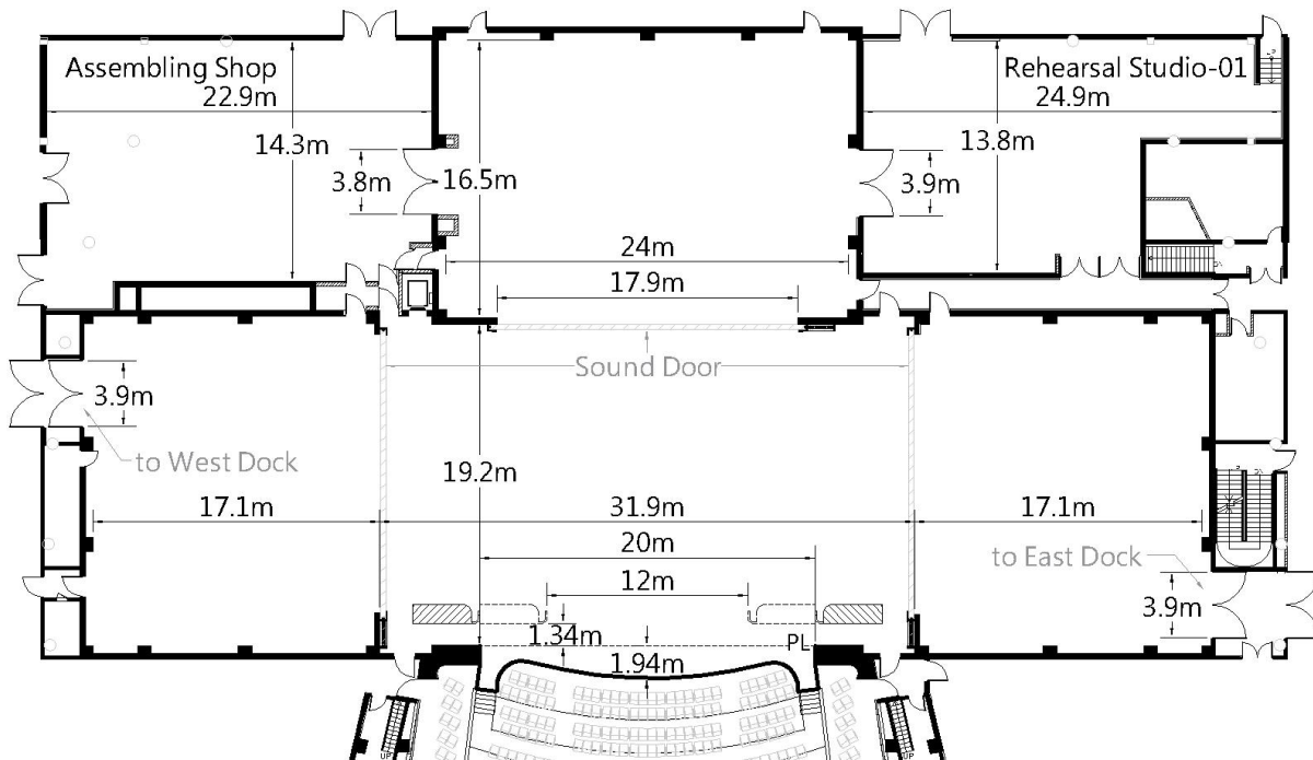
Figure 1.1.2- Stage Plan
