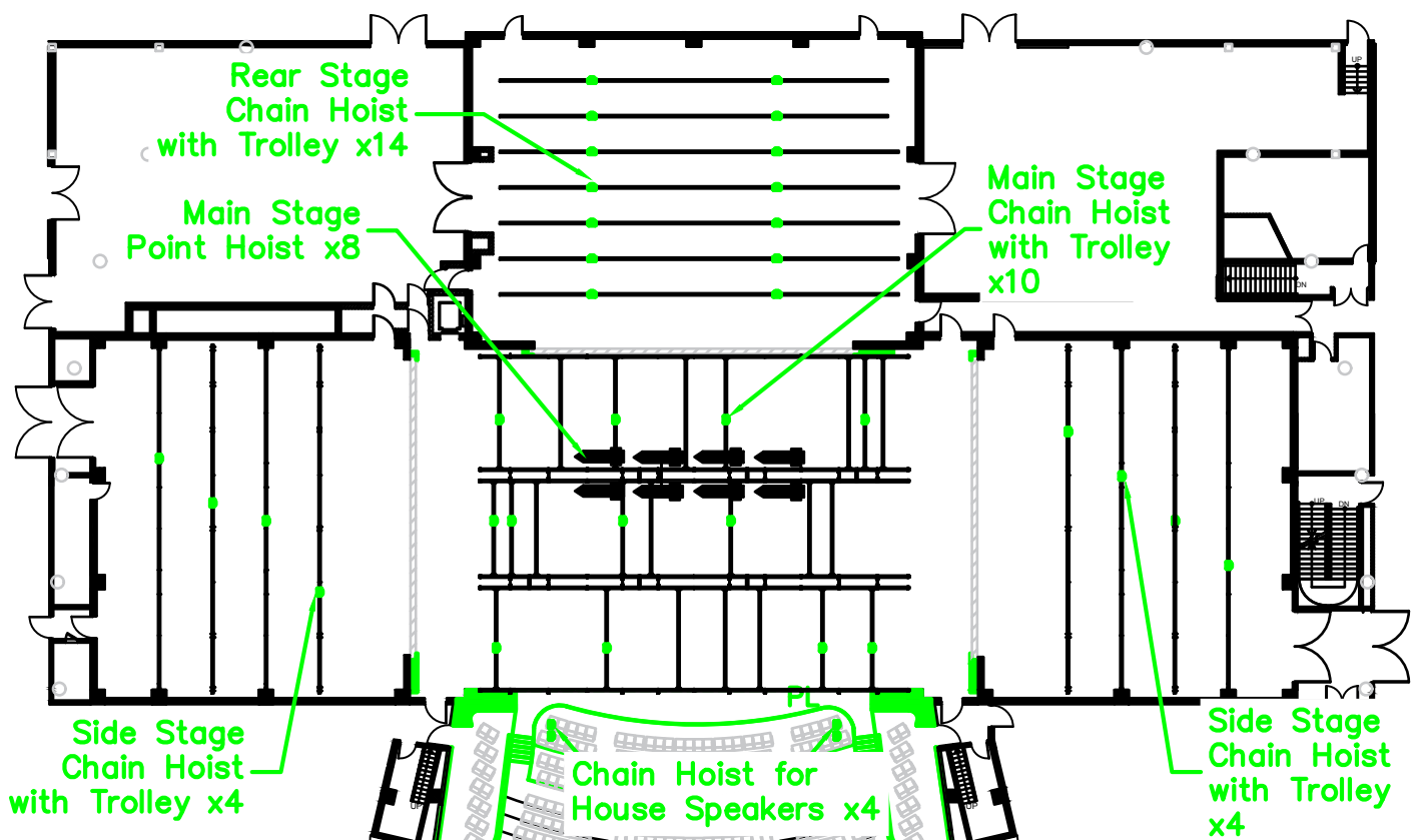
Figure 1.4.1- Hoisting plan
