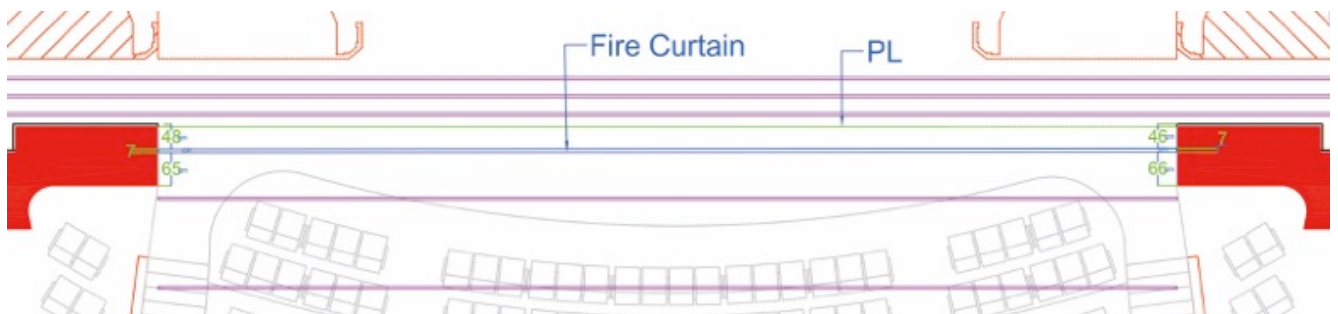
Figure 1.3.2- Fire Curtain
