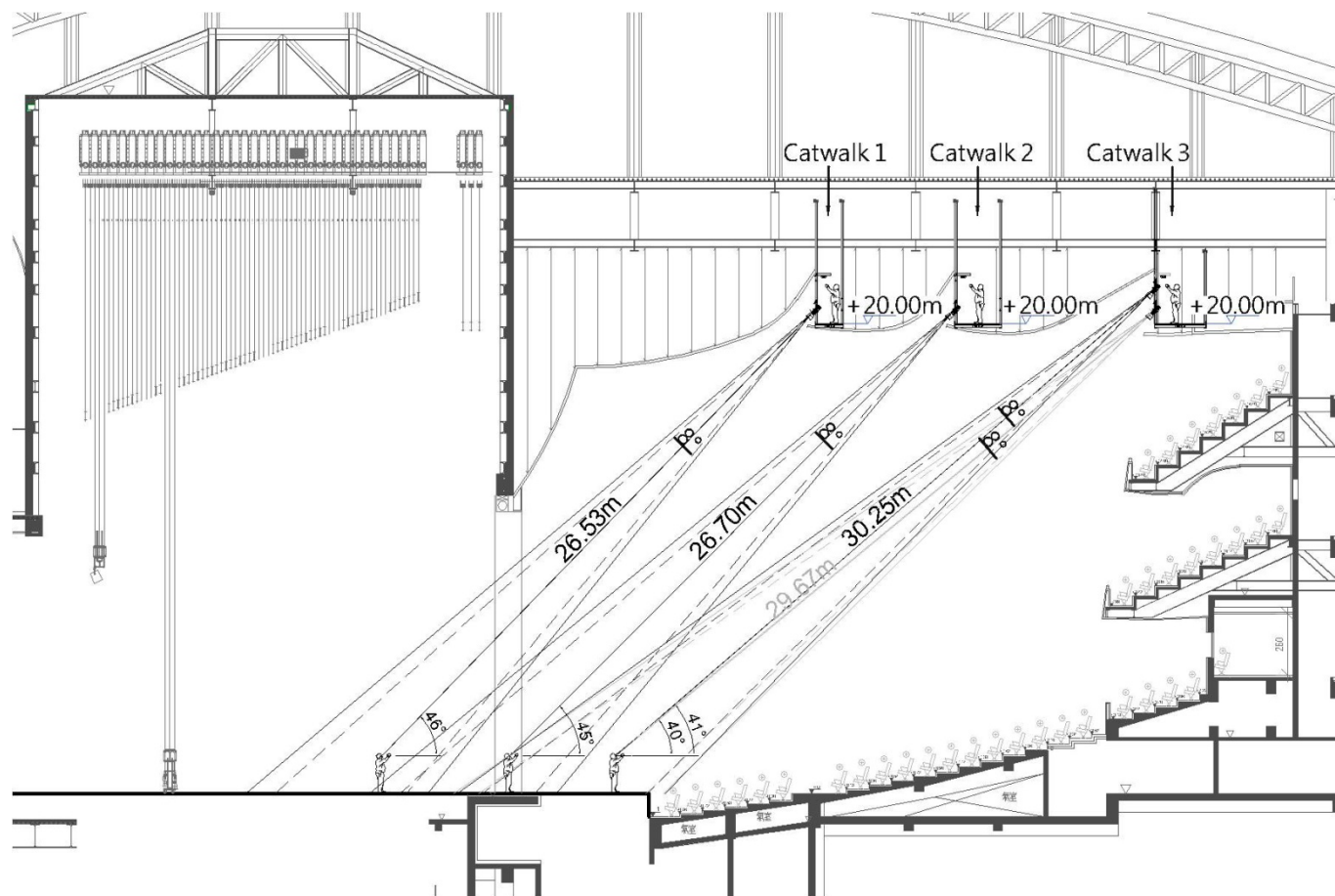
Figure 2.2- Lighting Section
